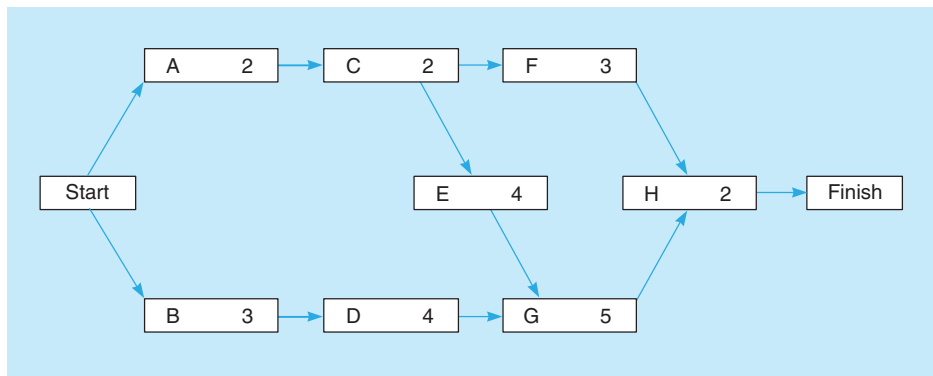
FIGURE 12.12 General Foundry's Network with Activity Times
