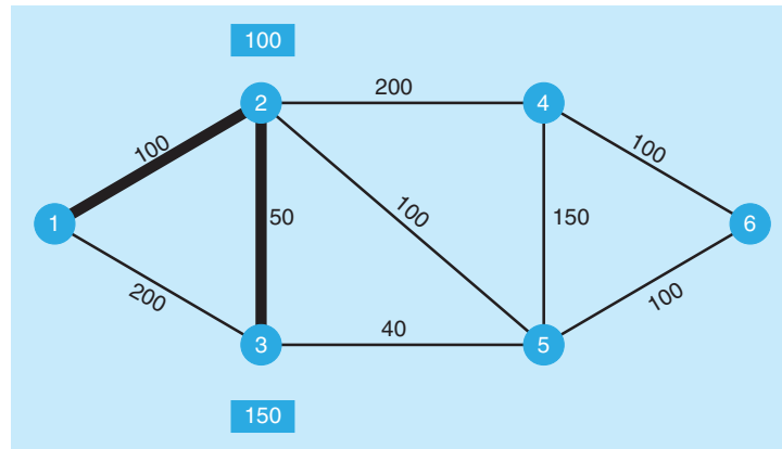
FIGURE 11.12 Second Iteration for Ray Design
