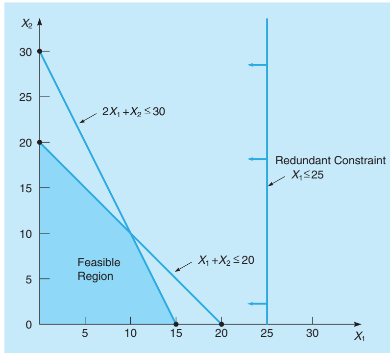
FIGURE 7.14 Problem with a Redundant Constraint
