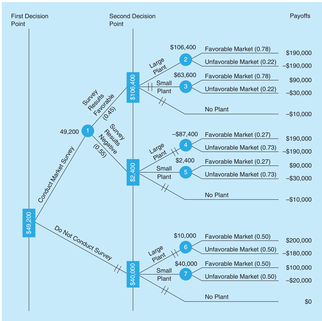
FIGURE 3.5 Thompson's Decision Tree with EMVs Shown
