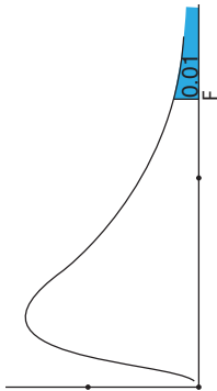
F distribution table for the upper 1% probability ( \alpha = 0.01 ).
