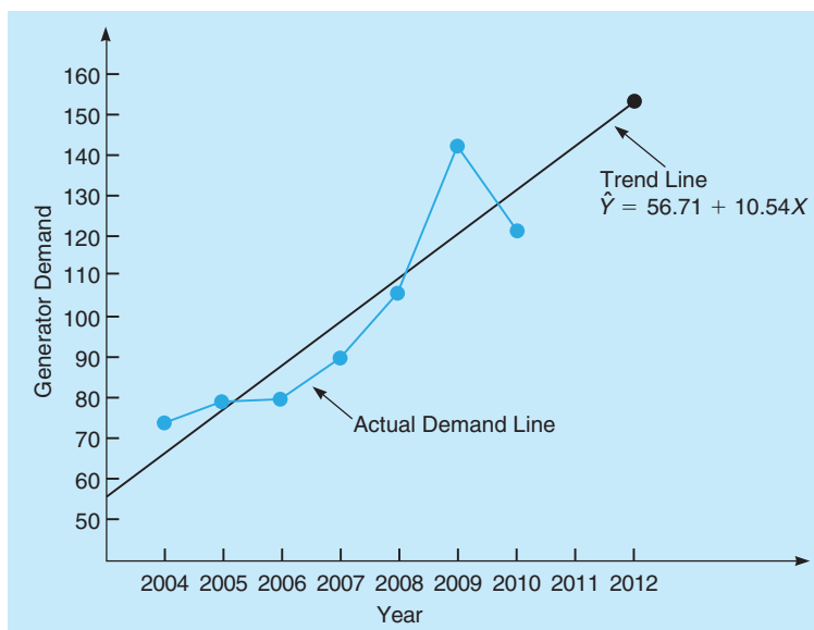
FIGURE 5.4 Electrical Generators and the Computed Trend Line
