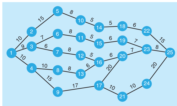
FIGURE 11.32 Network for Problem 11-36
