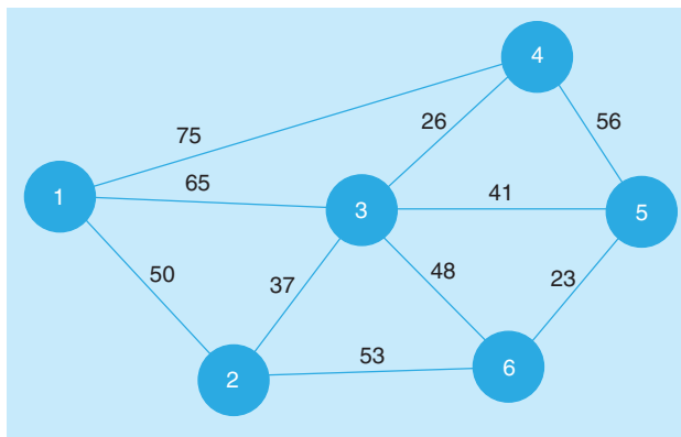
FIGURE 11.24 Network for Problem 11-14
