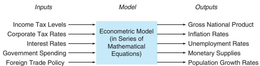
FIGURE 14.5 Inputs and Outputs of a Typical Economic System Simulation
