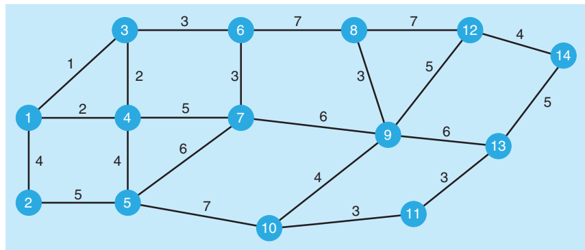
FIGURE 11.21 Network for Problem 11-9
