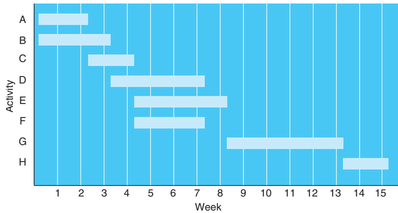
FIGURE 12.9 Gantt Chart for General Foundry Example
