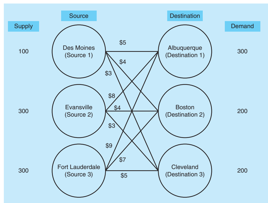
FIGURE 9.1 Network Representation of a Transportation problem, with Costs, Demands, and Supplies
