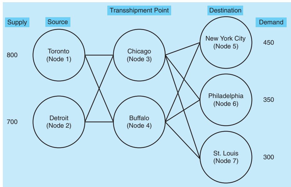
FIGURE 9.3 Network Representation of Transshipment Example
