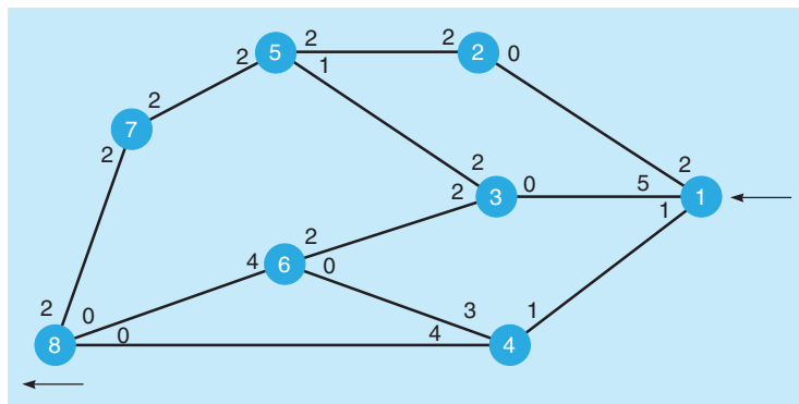
FIGURE 11.22 Network for Problem 11-10
