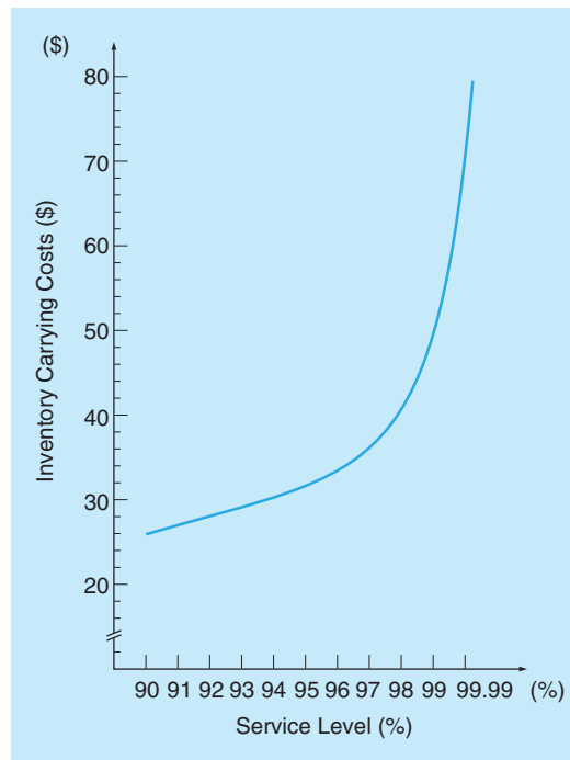
FIGURE 6.9 Service Level Versus Annual Carrying Costs
