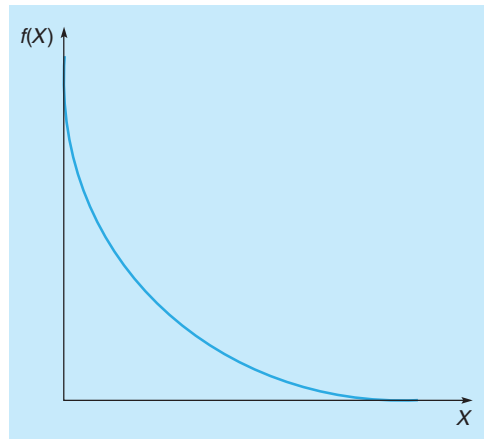
FIGURE 2.17 Exponential Distribution
