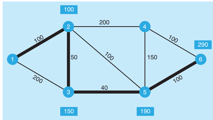
FIGURE 11.14 Fourth and Final Iteration for Ray Design
