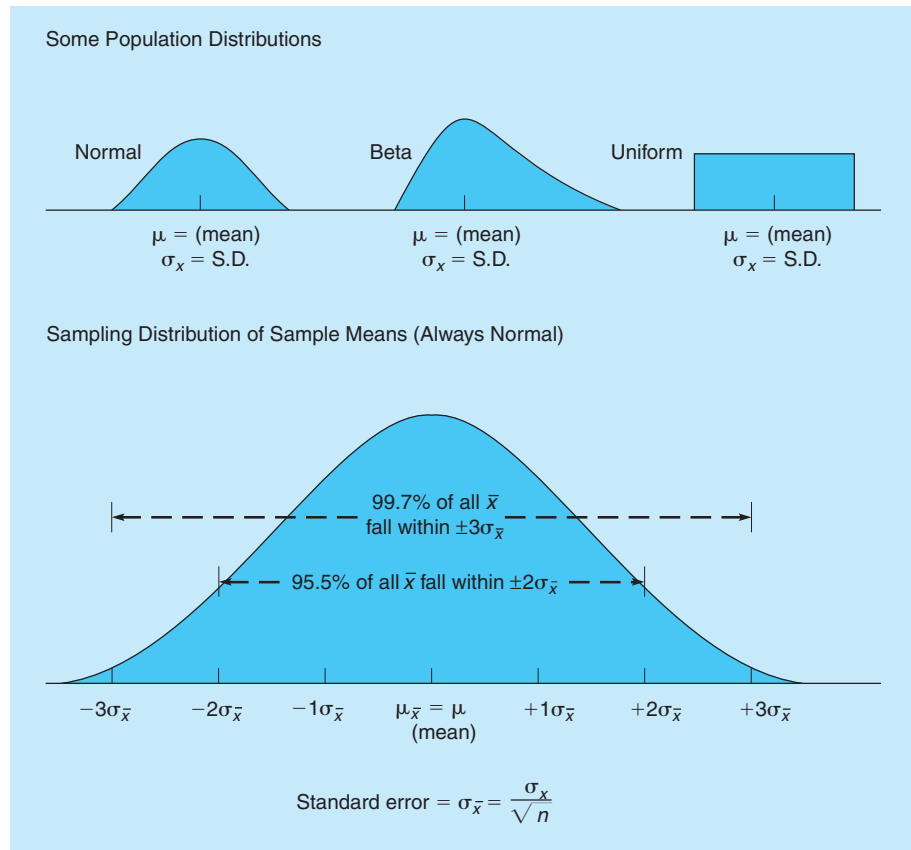
FIGURE 16.2 Population and Sampling Distributions
