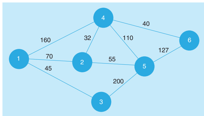
FIGURE 11.25 Network for Problem 11-15
