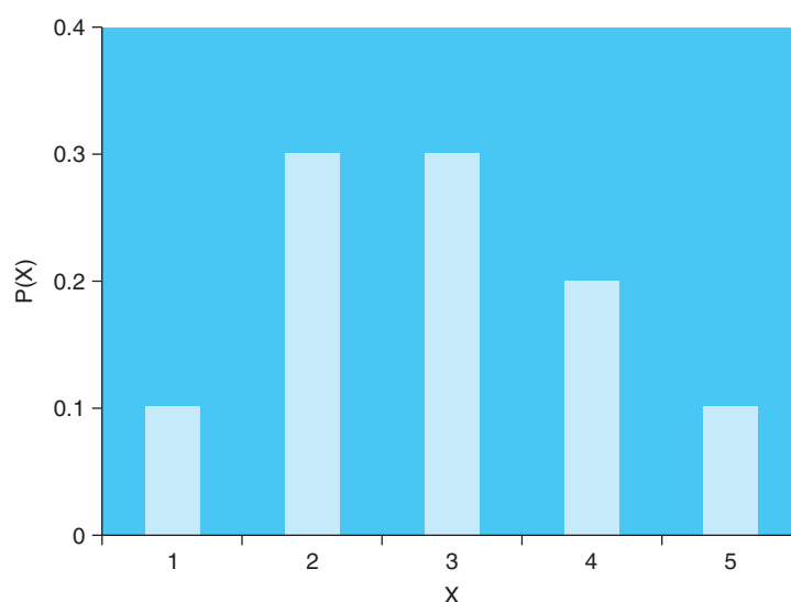
FIGURE 2.5 Probability Distribution for Dr. Shannon's Class
