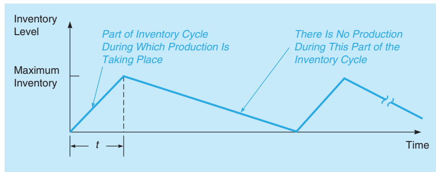
FIGURE 6.5 Inventory Control and the Production Process
