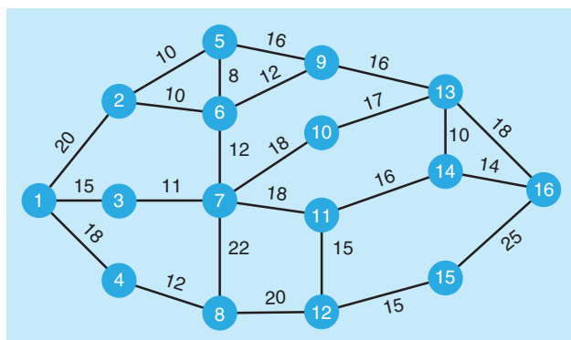
FIGURE 11.29 Network for Problem 11-25
