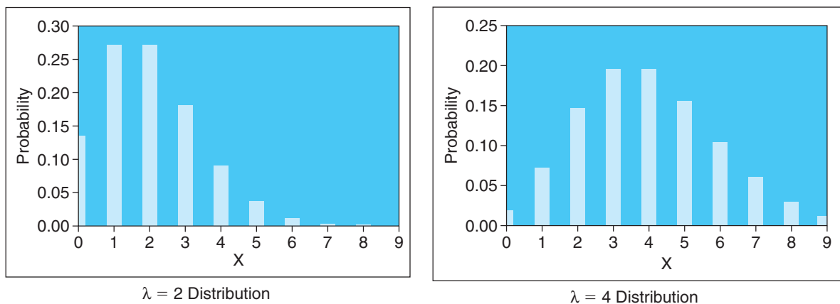
FIGURE 2.19 Sample Poisson Distributions with \lambda = 2 and \lambda = 4
