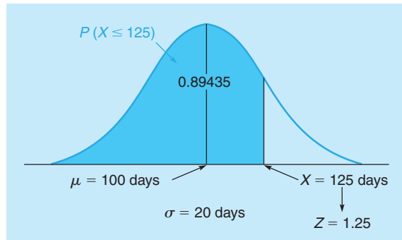
FIGURE 2.11 Normal Distribution for Haynes Construction
