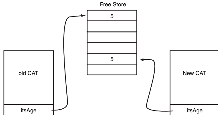
FIGURE 10.3 Deep copy illustrated.
