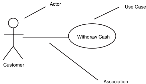
FIGURE 11.9 Use-case diagram.
