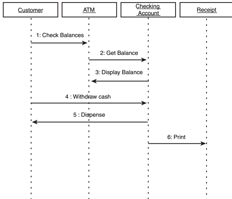
FIGURE 11.21 Sequence diagram.
