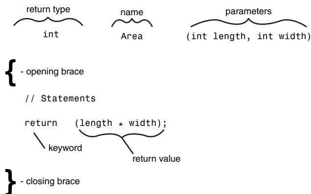
FIGURE 5.3 The header and body of a function.
