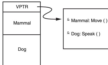
FIGURE 12.4 The v-table of a Dog.
