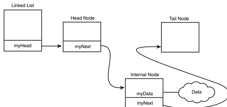
FIGURE E.3 The linked list after the first node is inserted.
