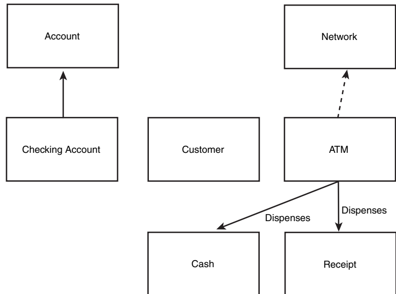
FIGURE 11.12 Preliminary classes.
