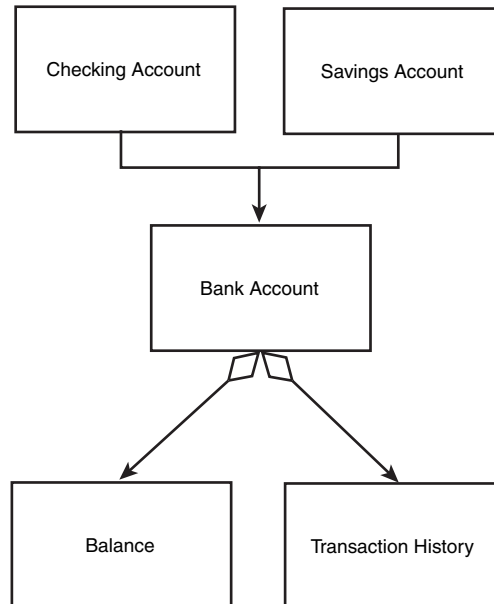
FIGURE 11.7 Object relationships.
