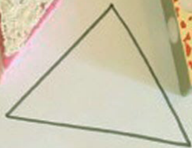
Triangle
