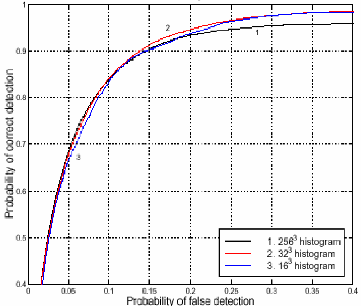
ROC curves on test set showing effect of increased bin size
